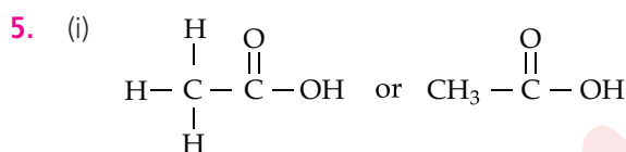
Ethanoic acid
