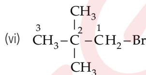
1-Bromo-2,2-dimethylpropane
