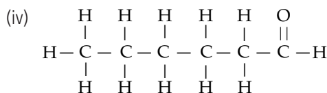
Hexanal
